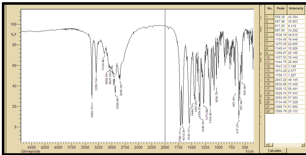
Figure No.4: FT-IR Spectra of Glimepiride
