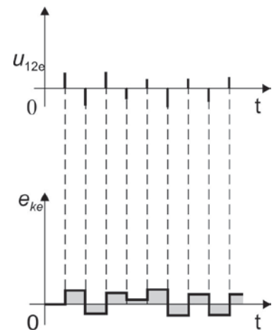
Picture 12: Procedure by item 9.2.1.2 – Earthing of the tank truck, through the proposed passive device for elimination of static electricity; Presentation of the state of earthing the tank truck model through the proposed passive device for elimination of static electricity. Now the values of voltage u_{12} = u_{12e} and one-way electromotor forces e_k = e_{ke} are smaller in time t , [1, 2].
