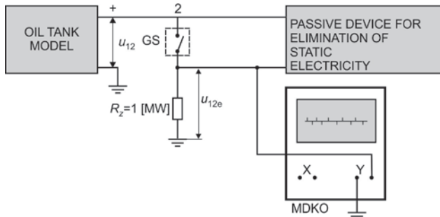
Fig. 10: Functional test of the efficiency of work of the passive device for elimination of static electricity (PU) in the laboratory and real conditions, by comparing results of elimination of static electricity obtained by earthing the tank truck through a cam switch (GS) and device (PU) on the oscilloscope (MDKO) [1,2].
