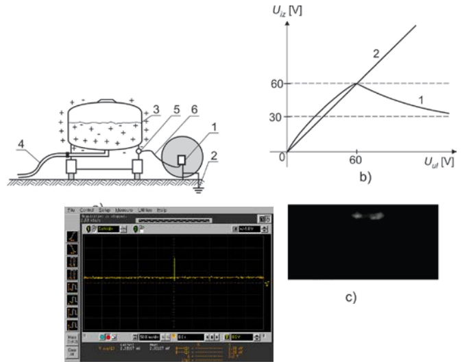
Fig. 13: Presentation of basic characteristics of the proposed and realized passive device for elimination of static electricity, PU [1, 2].
