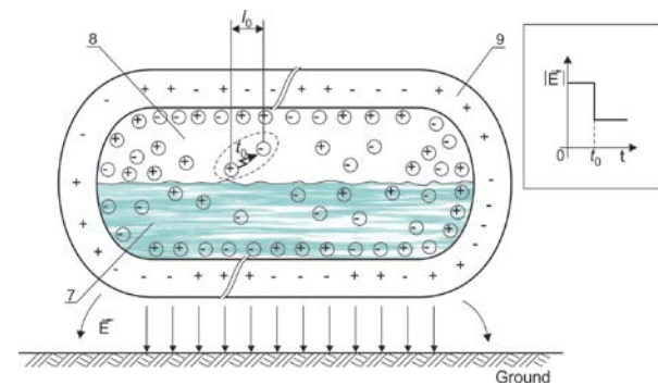
Picture 8: Planar (cross) section of the tank truck model in real conditions with adequate distribution of electricity, [1].
