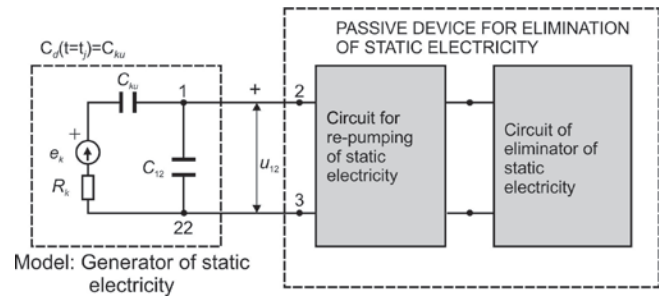
Fig. 9: Schematic presentation of the proposed passive device for elimination of static electricity connected to the source of the static electricity established in the borderline layer of the contact of the twofold layer of oil (or oil derivative) – inner metal wall of the tank truck model, [1, 2].
