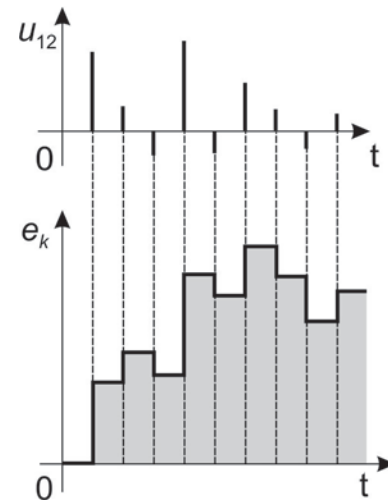
Picture 11: Procedure by item 9.2.1.1 – Earthing of the tank truck, directly through a cam switch; Presentation of the one-way electromotor force e_k of the equivalent generator of the tank truck model, while voltage is a differentiated value of e_k in time t , and in case of earthing the tank truck model through a cam switch (GS), presented in this picture, [1, 2].
