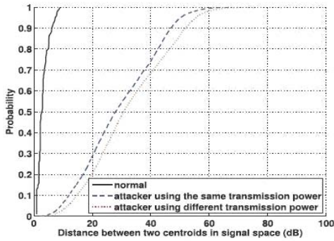
Fig-2: Different transmission power. [7]
