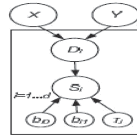
Fig 3: Bayesian graphical models. [7]
