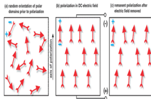
Fig:1. (a) Random orientation of domains prior to poling
