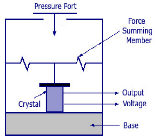
Piezo-Electric Transducer
