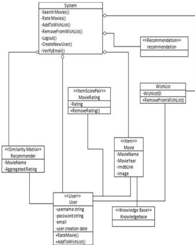
Fig. 4. Class diagram of case study
