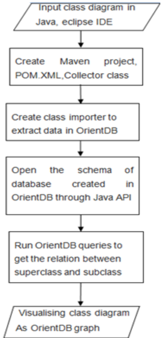
Fig. 5. Flowchart to represent class diagram in OrientDB
