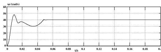
Figure 4.4 (b) SVM-DTC speed waveform
