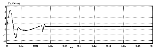
Figure 4.3 (b) SVM-DTC torque waveform
