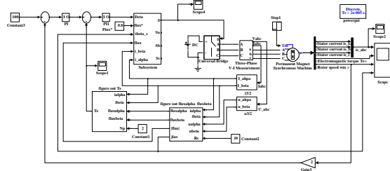
Figure 3.3.1 Permanent magnet synchronous motor SVM-DTC simulation model
