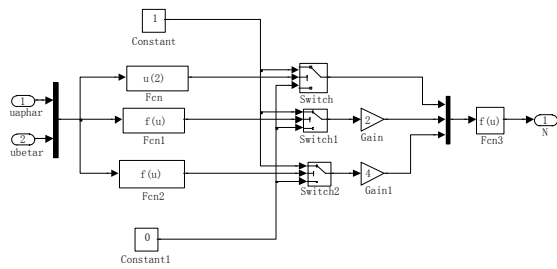
Figure 3.3.3 Calculation of the intermediate variable
