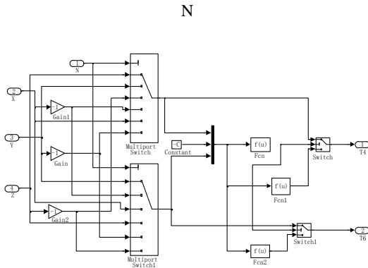
Figure 3.3.4 Calculation of the respective acting time T_4 , T_6 of the basic voltage space vector U_4 , U_6
