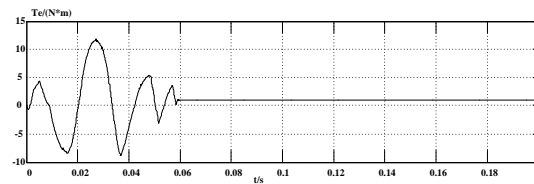
Figure 4.3 (a) DTC torque waveform
