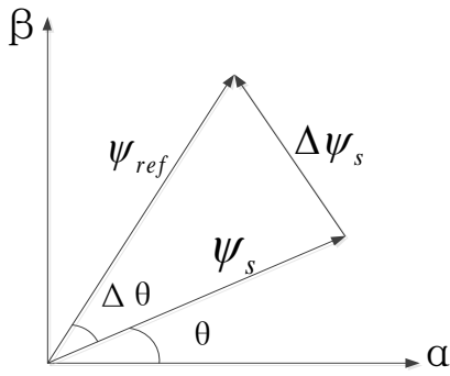
Figure 3.2.1 Stator flux vector
