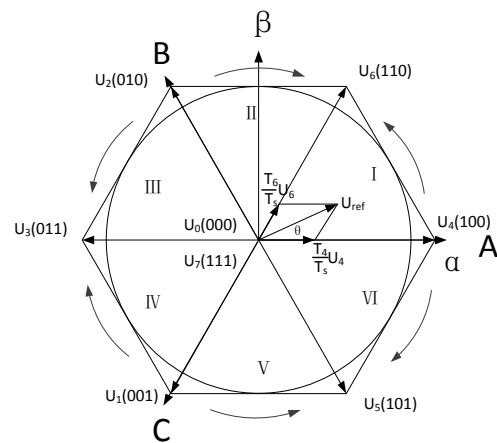
Figure 3.2.2 Reference voltage space vector synthesis diagram
