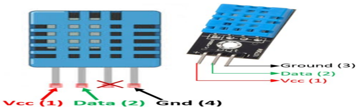
Figure 1: Temperature and Humidity sensor DHT11
