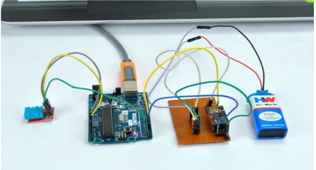
Figure 3: Arduino Uno board with 9V DC power supply
